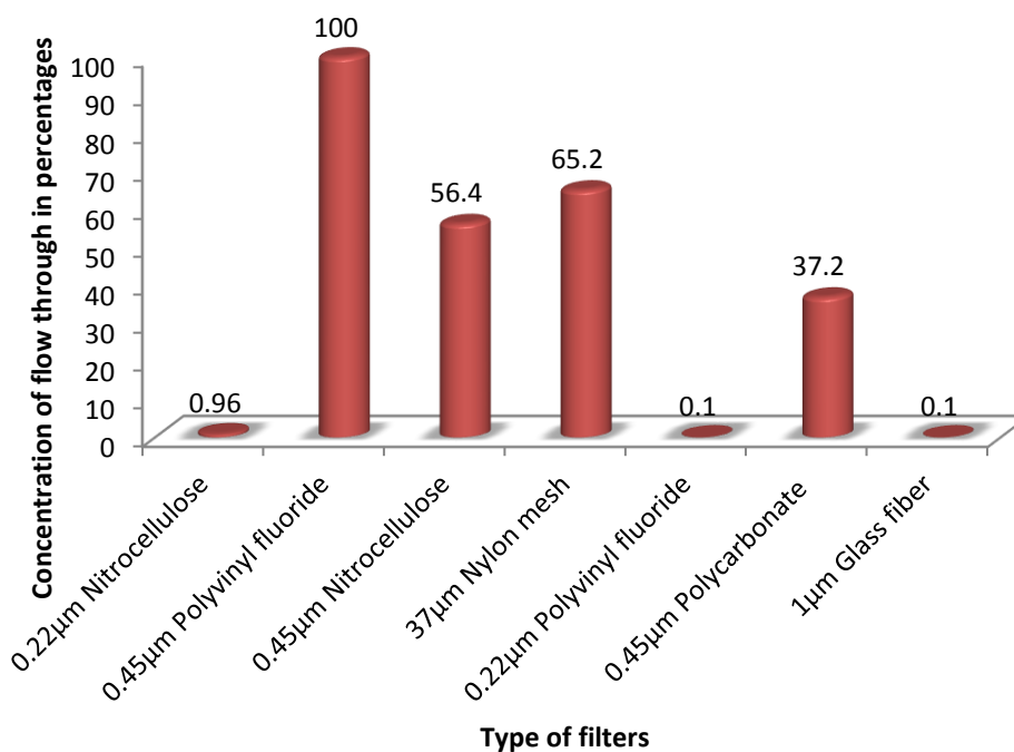
Fig. 2: Average percentage of leptospire in cultures that were found in filtrate with 95% confidence intervals displayed
